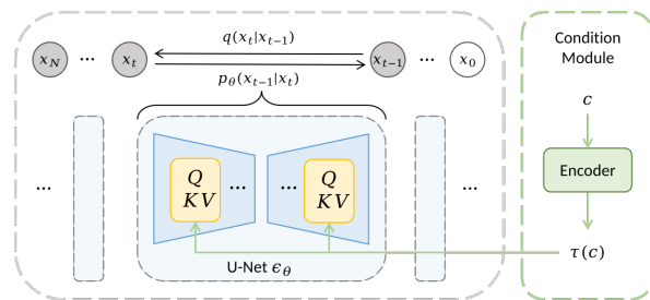
Figure 2: The model structure with an additional condition module for external control. Each UNet unit e_\theta applies one denoising step during the reverse process. External condition signals are encoded by pre-trained encoders and fed into the cross-attention layers, which are represented by the yellow squares in the UNet unit.
